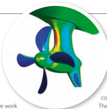
ABOVE: The two Azipull thrusters use large diameter propellers with a low blade area of very efficient shape.
